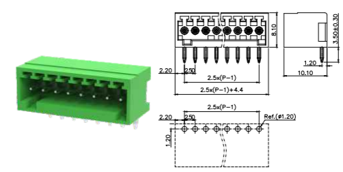
MC-DPA2.5HXX
