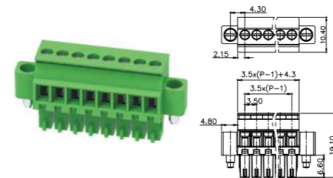
MC-RE3.5VXXC-RK-0001
