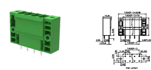
MC-PH7.62VXX-F
