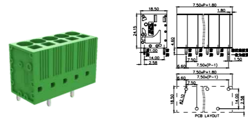
MC-TC7.5VXXP-Z-0001
