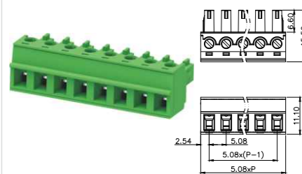
MC-RA5.08HXXC-0001
