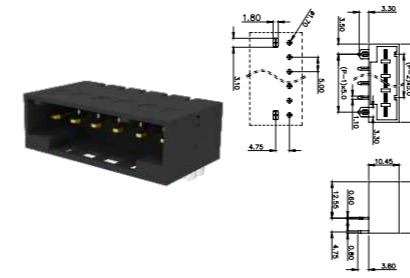
MC-POX5.0HXX-0001
